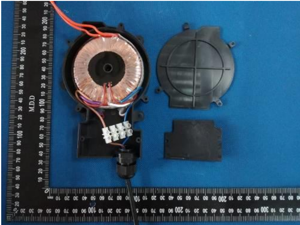
Photo 9 Internal view for model HX302401250Q2E-B
