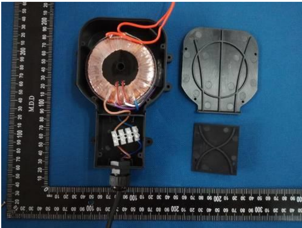
Photo 3 Internal view for model HX302401250Q2E-A
