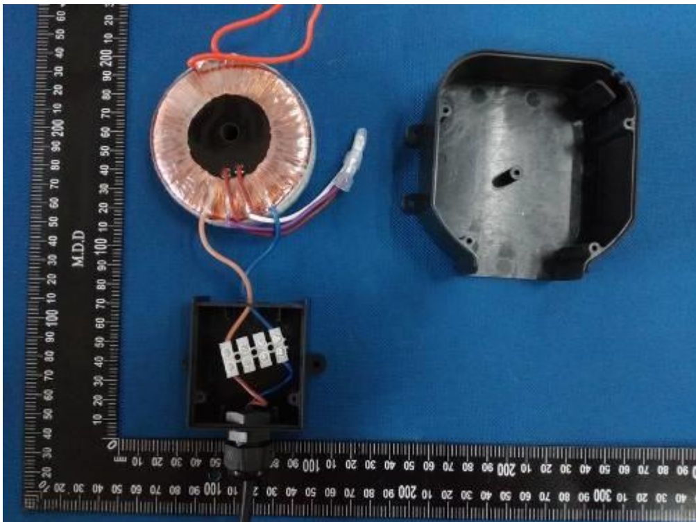
Photo 4 Internal view for model HX302401250Q2E-A
